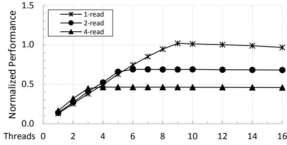
Fig. 6: 1\mu\text{s} prefetch-based access at various levels of MLP. Each line is normalized to the corresponding DRAM baseline.
