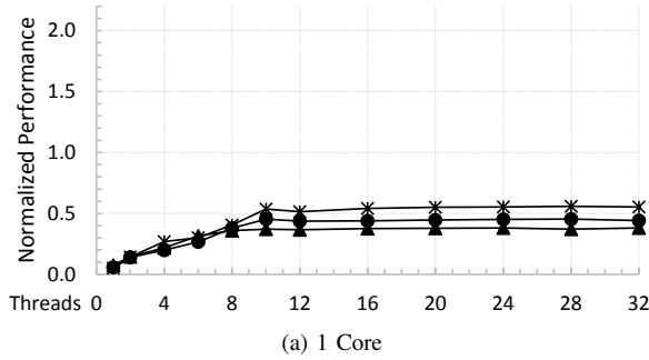
Fig. 9: Impact of MLP on software-managed queues with one and four cores. Each line is normalized to the corresponding DRAM baseline.
