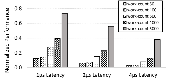
Fig. 2: On-demand access of microsecond-latency device. The values are normalized to the single-threaded on-demand DRAM baseline.
