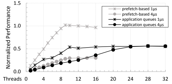
Fig. 7: Comparison of the application-managed queues and prefetch-based accesses with 1\mu\text{s} and 4\mu\text{s} device latencies.
