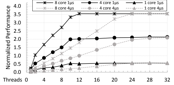
Fig. 8: Multicore comparison of software-managed queues with 1\mu\text{s} and 4\mu\text{s} device latencies.
