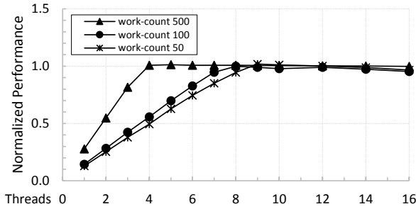
Fig. 4: 1μs prefetch-based access with various work counts. The values are normalized to the single-threaded on-demand DRAM baseline.
